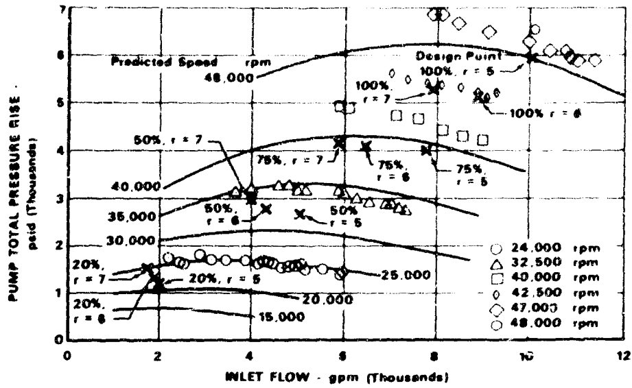
Figure 729. Pump Total Pressure Rise vs Inlet Flow, Rig 35147-1A FD 41270
