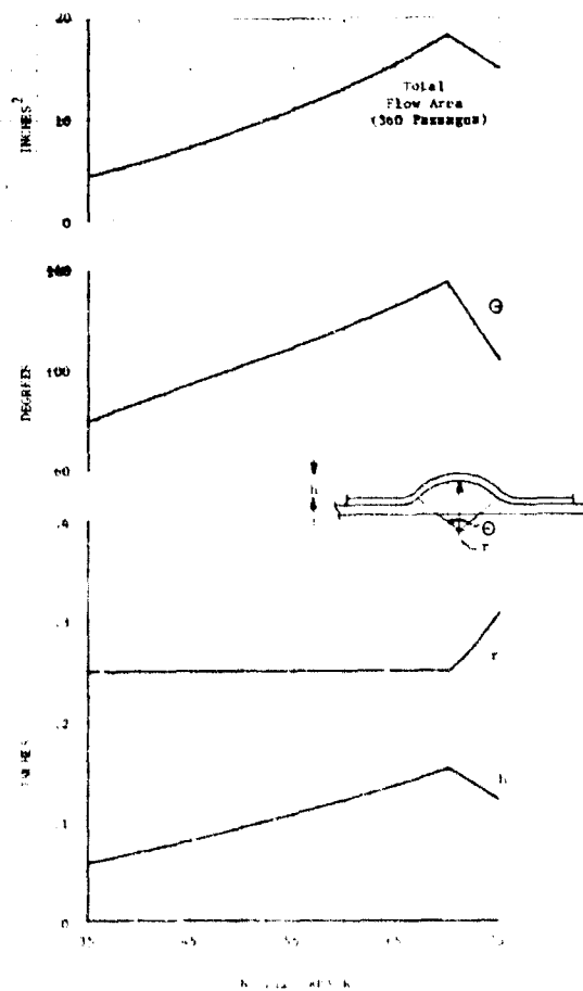
Figure 555. Two-Position Nozzle Geometry
