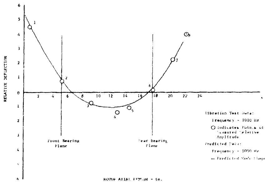
Figure 644. XLR129 Fuel Pump Rotor, Second Bending Mode Predicted and Test Results DF 76519
