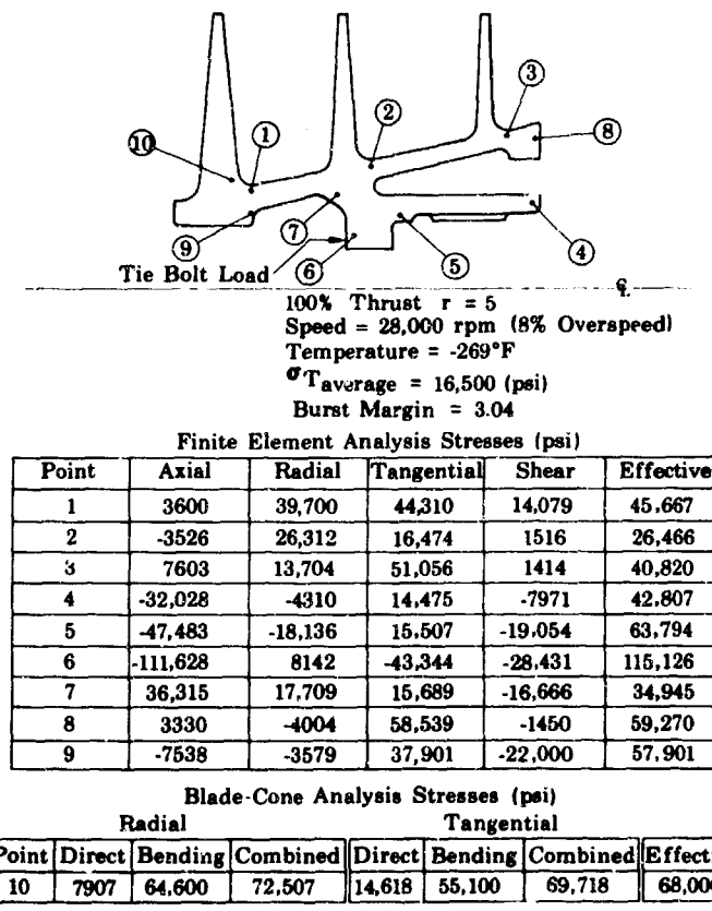
Figure 744. Oxidizer Turbopump High-Speed Inducer Stresses FD 33093
