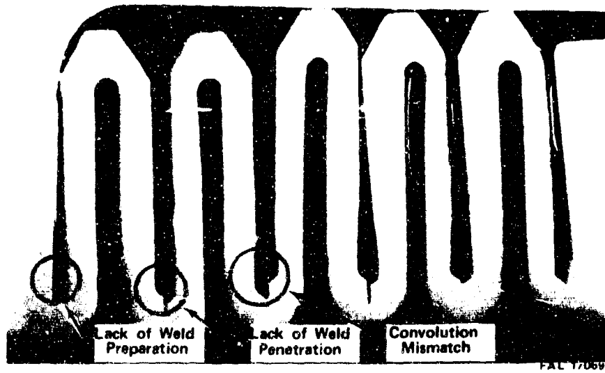
Figure 637. Inner Bellows Section Showing Fabrication Problem Areas
