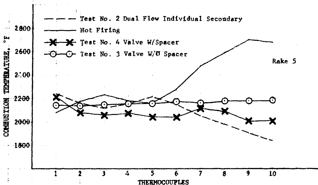
Figure 409. Combustion Temperature
