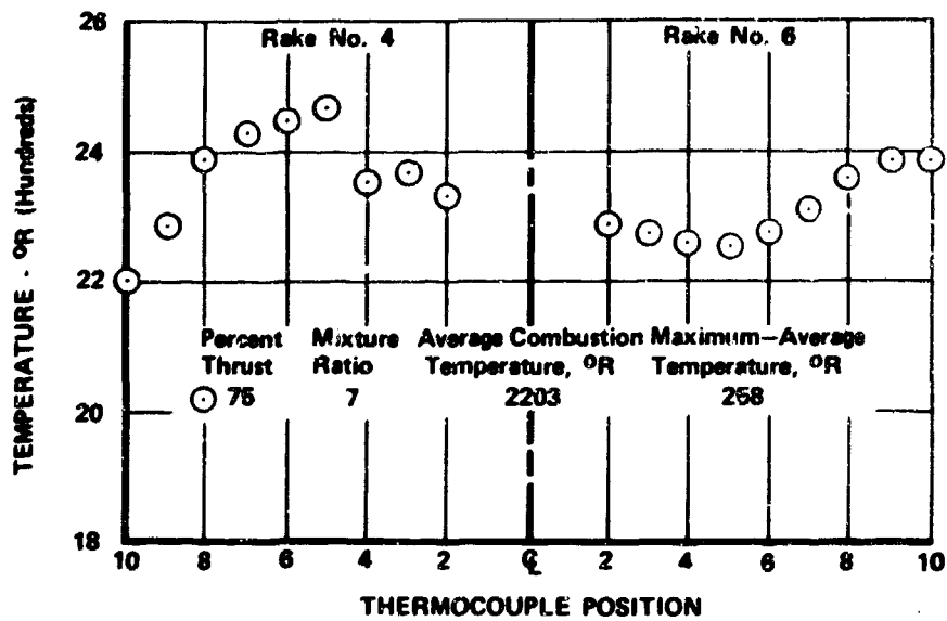
Figure 460. Temperature Distribution During Run 8.01
