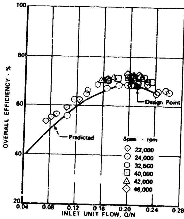
Figure 712. Overall Efficiency vs Inlet Unit Flow, Rig 35138-2
