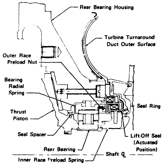
Figure 575. Rear Bearing and Mount Assembly FD 31623A
