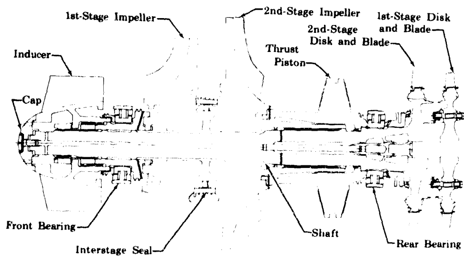
Figure 572. Rotor Assembly
