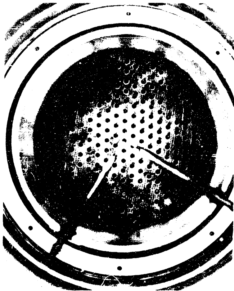
Figure 386. Injector Face Showing Good Condition Without Metal Erosion FE 89765
