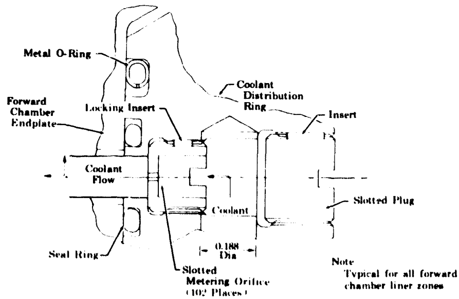
Figure 535. Forward Chamber Liner Coolant Metering Installation, Side View FD 31364
