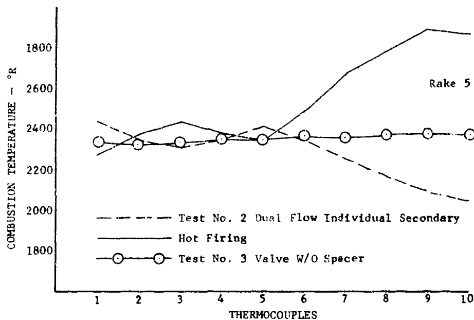
Figure 407. Combustion Temperature
