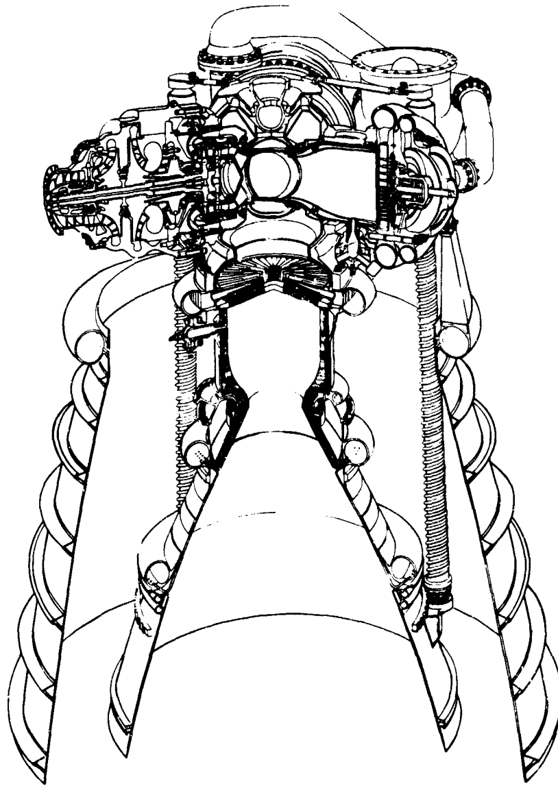
Figure 543. Location of Two-Position Nozzle and Translating Mechanism
