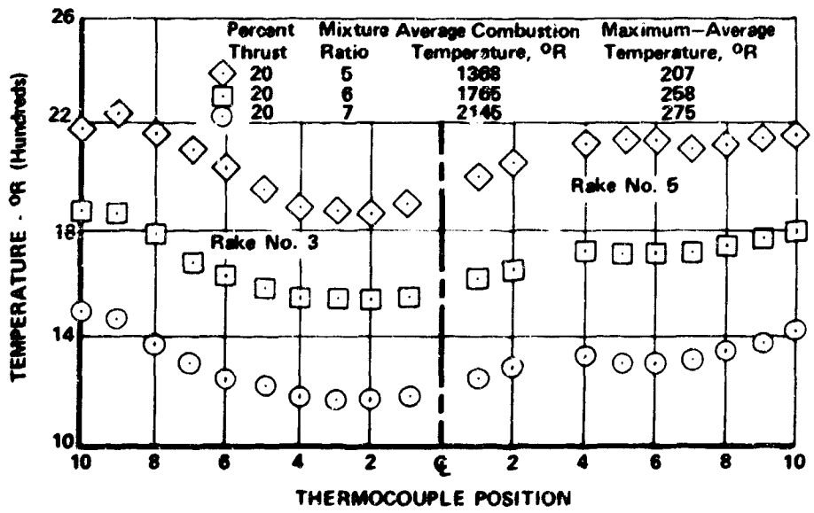
Figure 453. Temperature Distribution During Run 5.01
