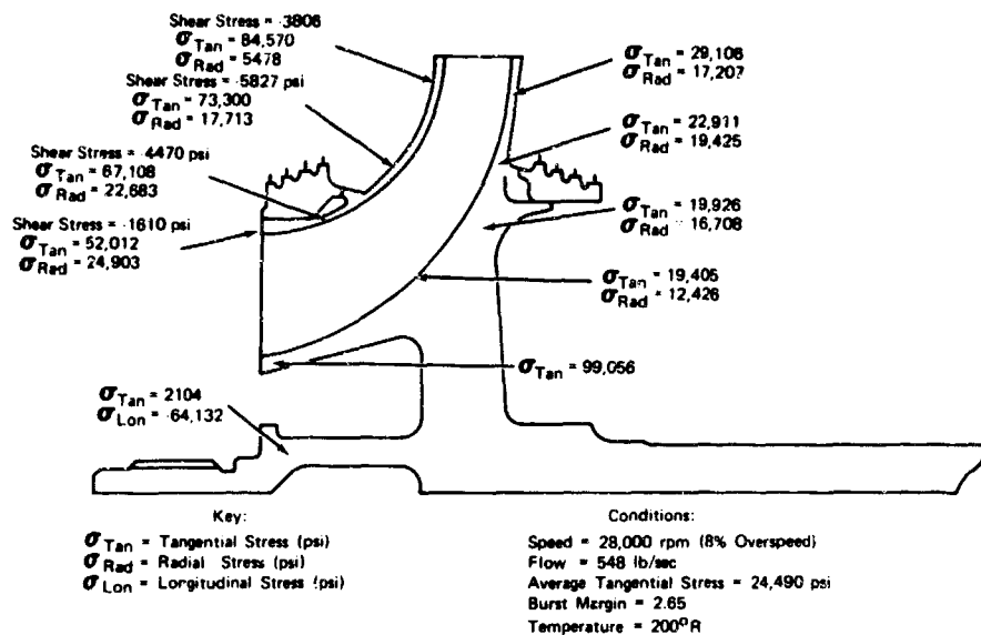
Figure 746. Oxidizer Turbopump Impeller Stresses FD 33095
