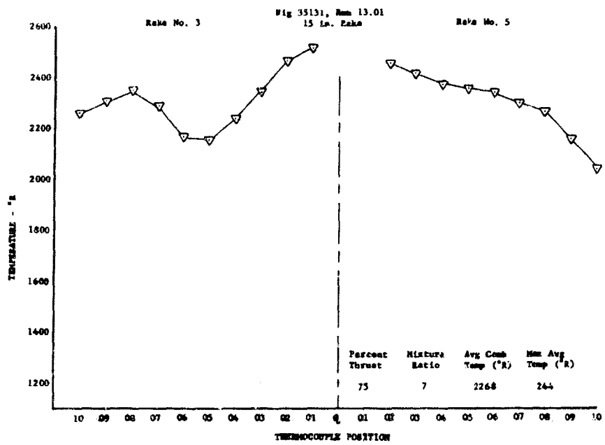
Figure 431. Fixed Area Preburner Temperature Profile, Run 13.01 DF 79869
