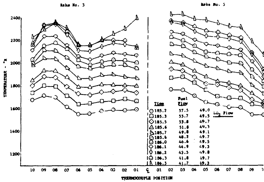
Figure 433. Fixed Area Preburner Temperature Profile, Run 13.01
