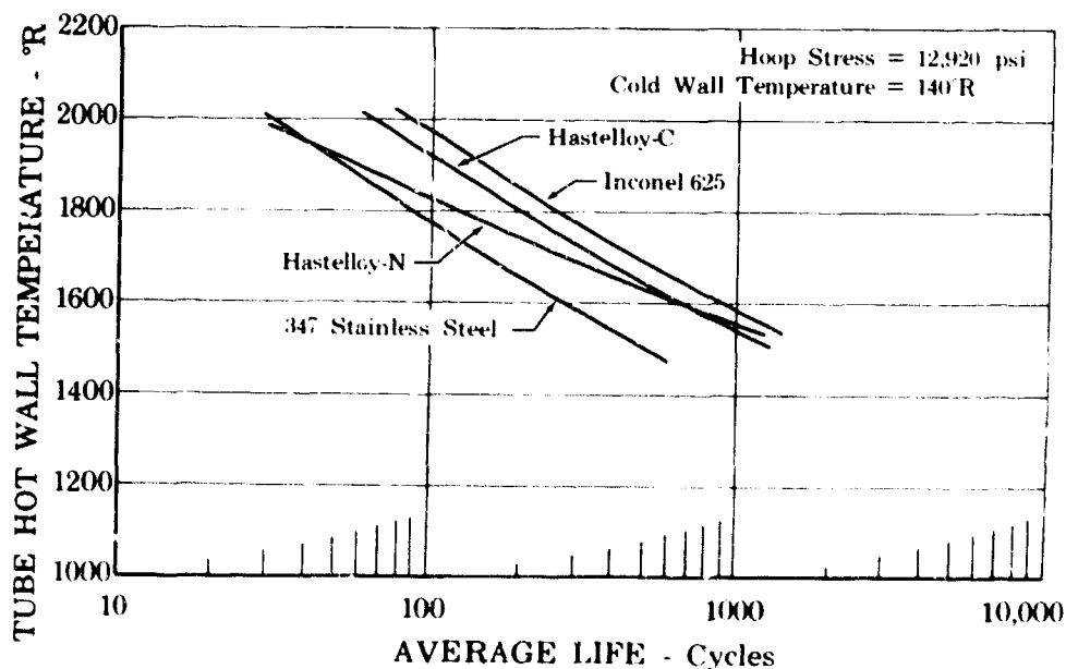
Figure 561. Inconel 625 Provides Highest Average Cycle Life FD 21090
