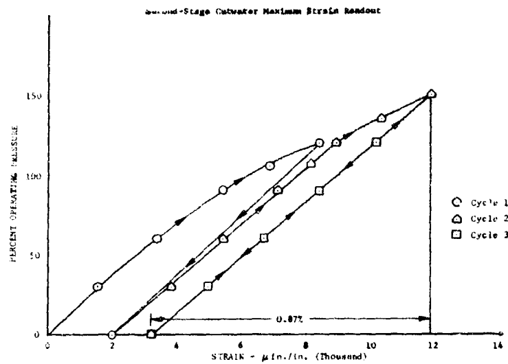
Figure 633. 2nd-Stage Cut Water Maximum Strain Readout
