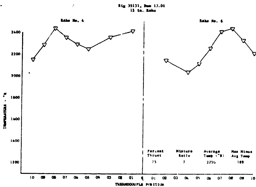
Figure 430. Fixed Area Preburner Temperature Profile, Run 13.01 DF 79868
