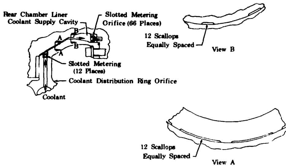
Figure 536. Rear Chamber Liner Coolant
