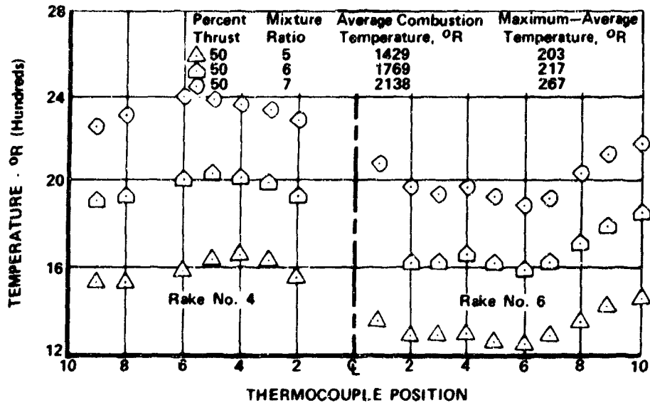
Figure 450. Temperature Distribution During Run 5.0i
