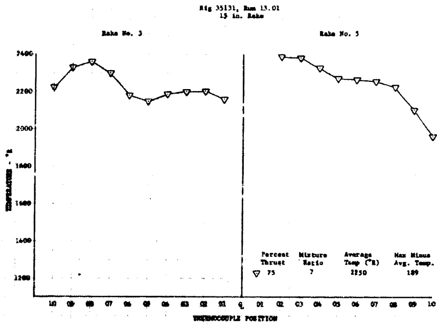
Figure 429. Fixed Area Preburner Temperature Profile, Run 13.01 DF 79867
