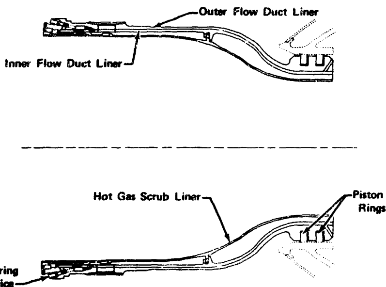
Figure 480. Preburner Flow Duct
