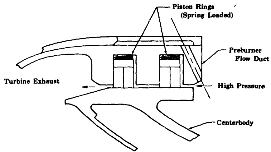
Figure 481. Preburner Flow Duct to Centerbody Piston Ring Connection
