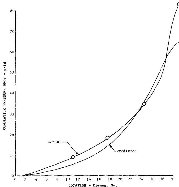
Figure 525. Comparison of Predicted and Actual Flow Data DF 70088
