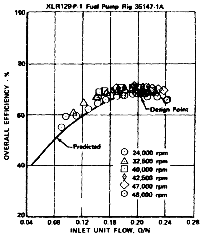
Figure 730. Overall Efficiency vs Inlet Unit Flow, Rig 35147-1A FD 41271
