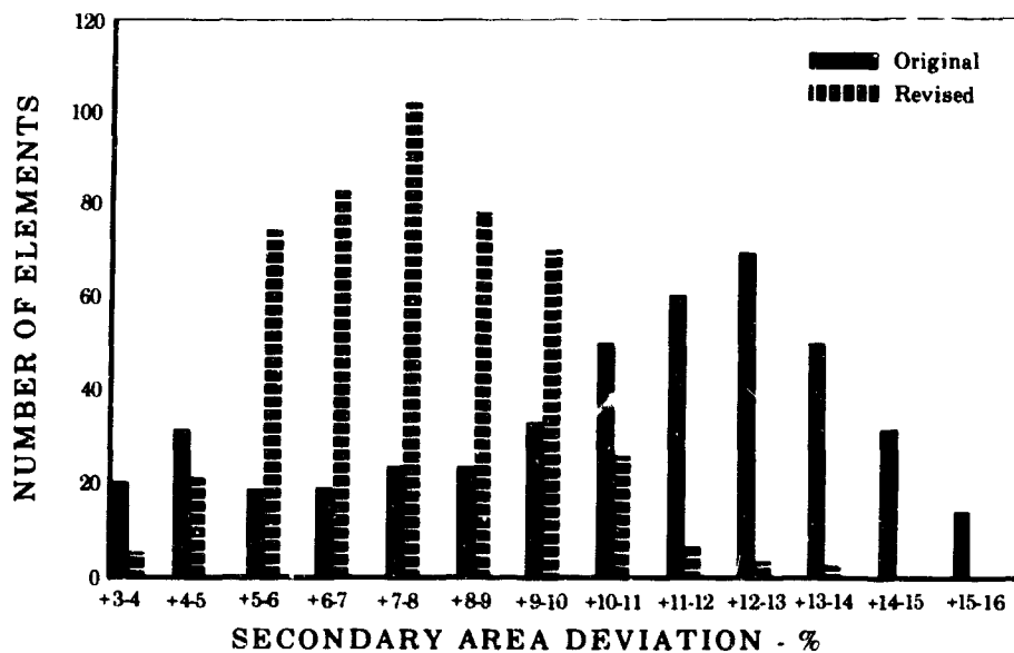
Figure 359. Preburner Injector Element Secondary Flow Area Deviations FD 29189
