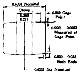
Figure 569. Roller Bearing Configuration
