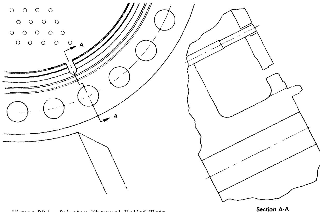
Figure 394. Injector Thermal Relief Slots
