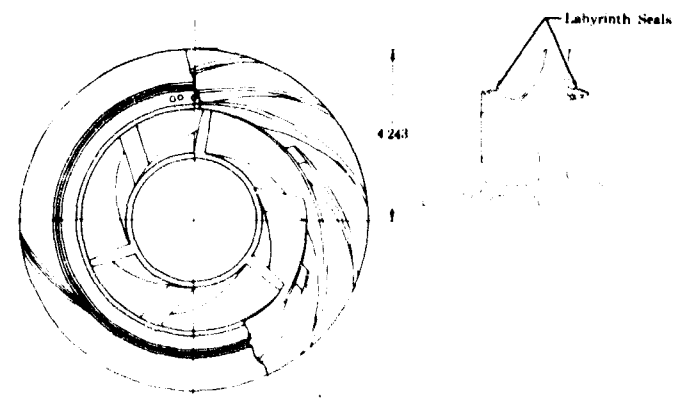
Figure 745. Oxidizer Turbopump Impeller FD 33094
