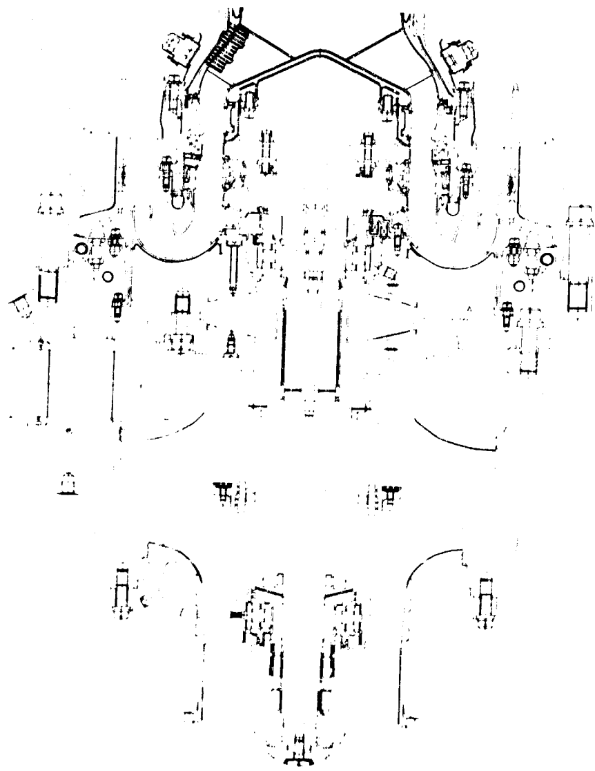
Figure 565. Fuel Turbopump Assembly
