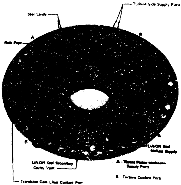
Figure 609. Rear Bearing Support and Rear Thrust Piston Housing - Front Side Up FD 38337
