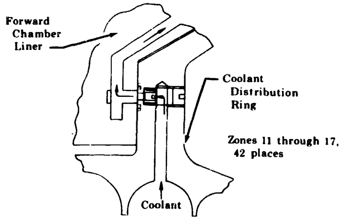
Figure 534. Forward Chamber Coolant Metering FD 31367
