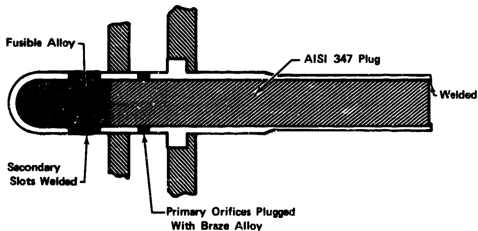
Figure 415. Six Elements With Blocked Primaries Plugged By Welding
