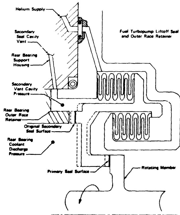
Figure 578. Fuel Turbopump Lutoff Seal
