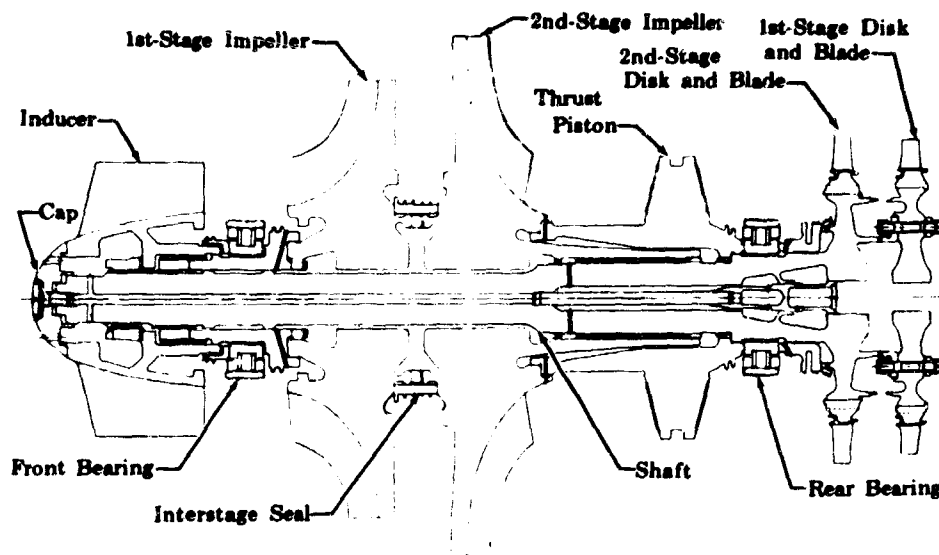
Figure 588. Rotor Assembly
