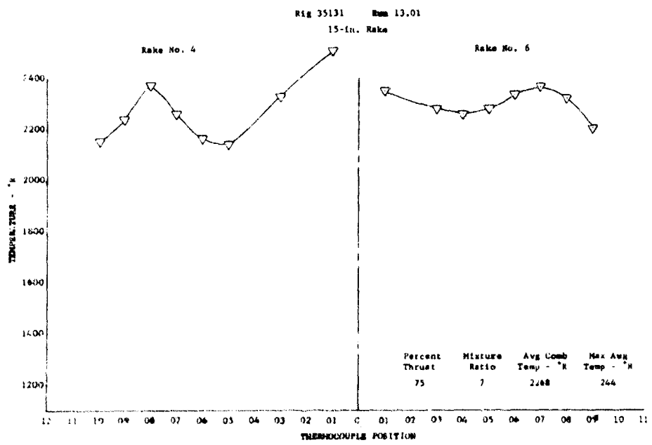
Figure 432. Fixed Area Preburner Temperature Profile, Run 13.01 DF 79870
