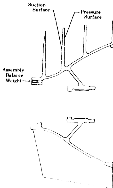
Figure 776. Oxidizer Inducer
