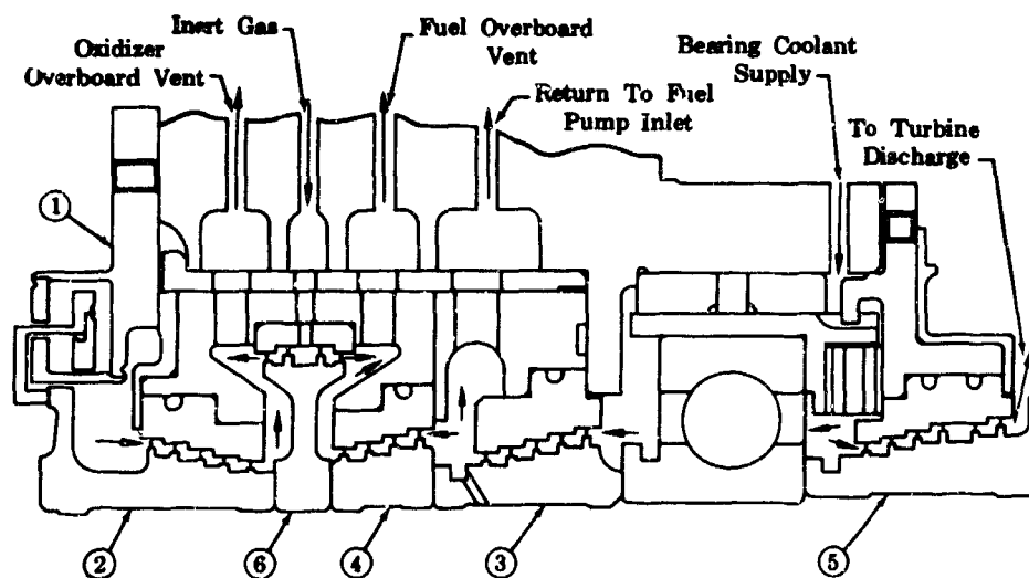
Figure 753. Oxidizer Turbopump Seal Package
