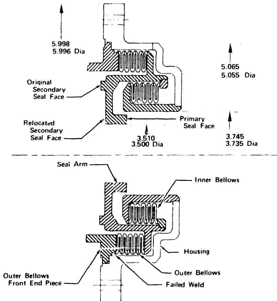
Figure 636. Cross Section of Lutoff Seal Assembly
