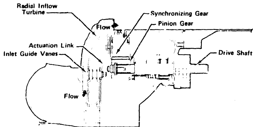
Figure 778. Oxidizer Low-Speed Inducer Turbine and Variable Guide Vanes FD 33337B
