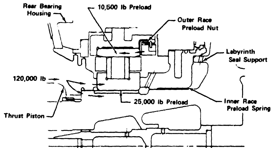
Figure 576. Rear Bearing Preloading FD 31552A
