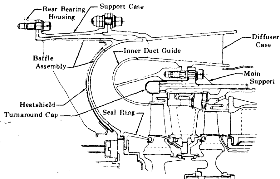
Fig. 586. Turbine Discharge Turnaround Manifold
