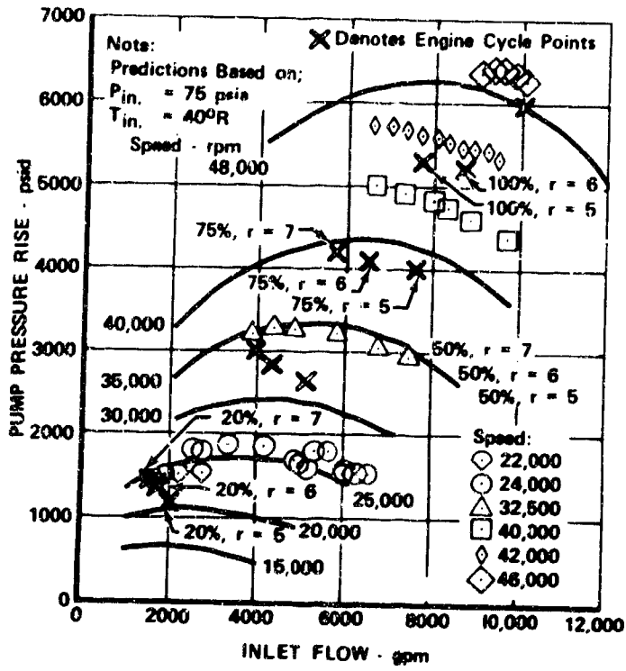
Figure 711. Pump Pressure Rise vs Inlet Flow, Rig 35138-2
