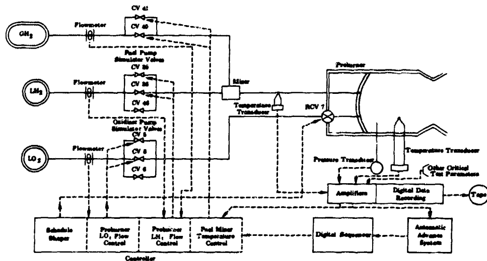
Figure 474. Preburner Rig Control System
