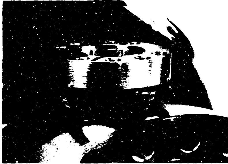
Figure 498. Advanced Propulsion XLR129 Preburner Outer Case Showing Locations of Strain Gage Rosettes No. 45 and 46. (2147902 S/N 1) FMDL 14837-10
