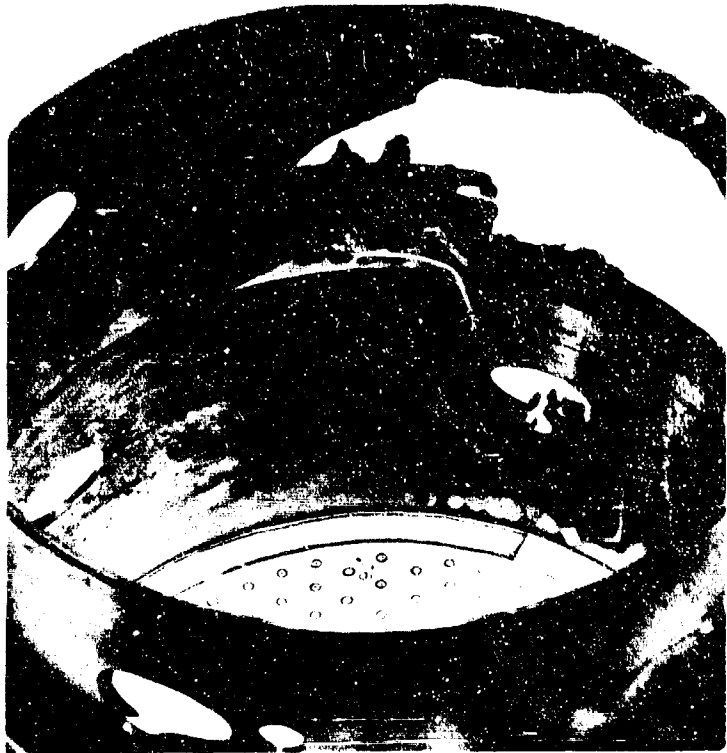
Figure 389. Scrub Liner Burning Pattern, 90 deg View
