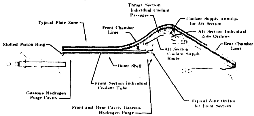
Figure 531. Main Burner Chamber Assembly, Side View FD 31972A
