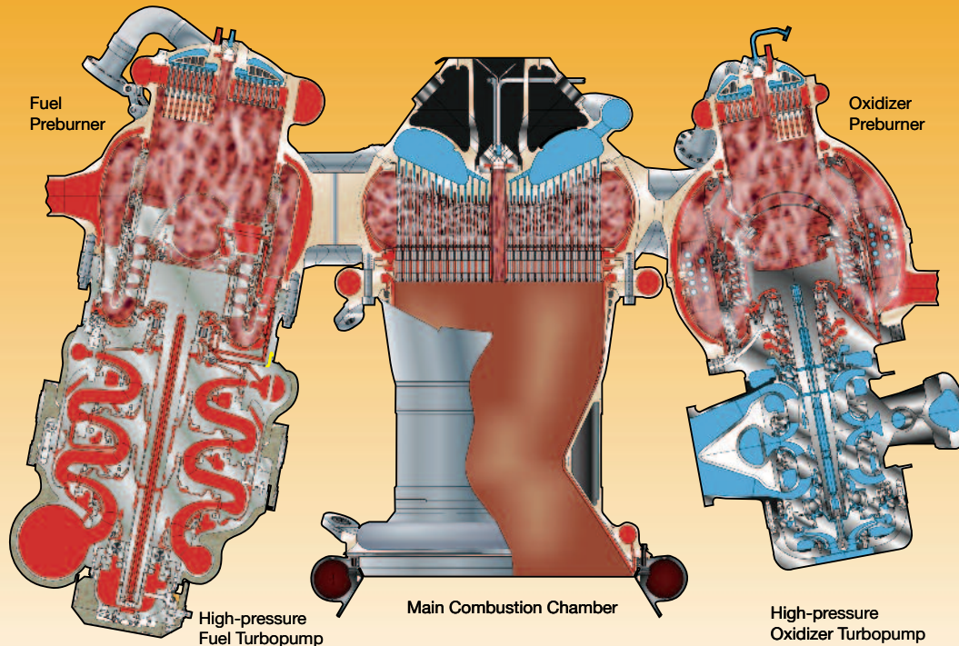
The Block II engine combined a new high-pressure fuel turbopump with the previously flown redesigned high-pressure oxygen turbopump. Risk analysis showed that the Block II engine was twice as safe as the 1990s-era engine. Beginning with STS-110 in April 2002, all shuttle flights were powered by the improved Space Shuttle Main Engine.
