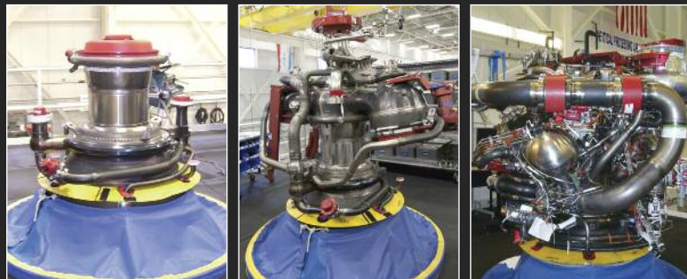
Space Shuttle Main Engine assembly.
