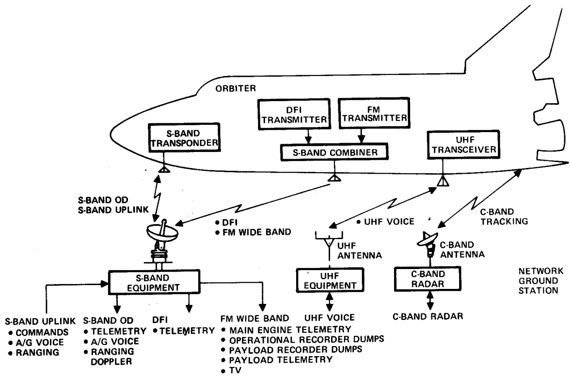
Figure 1. Orbiter-to-Ground Data Links
