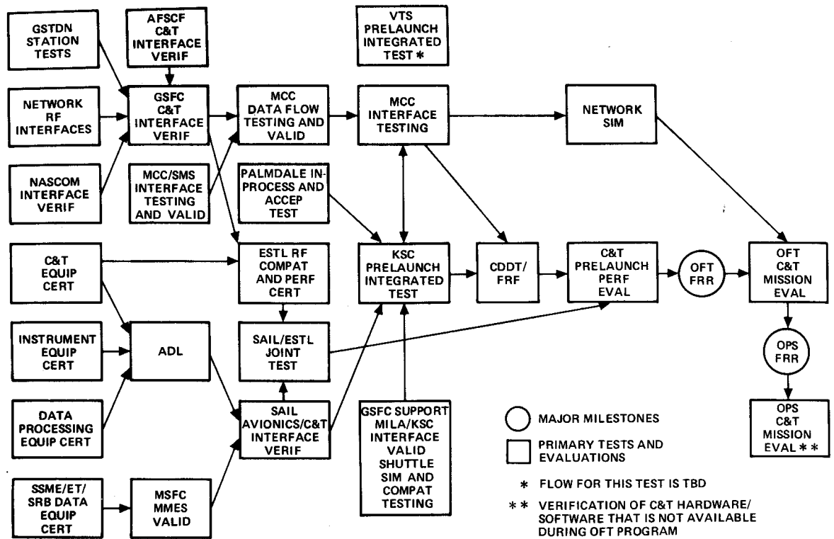
Figure 2 Communications and Tracking System Verification Network
