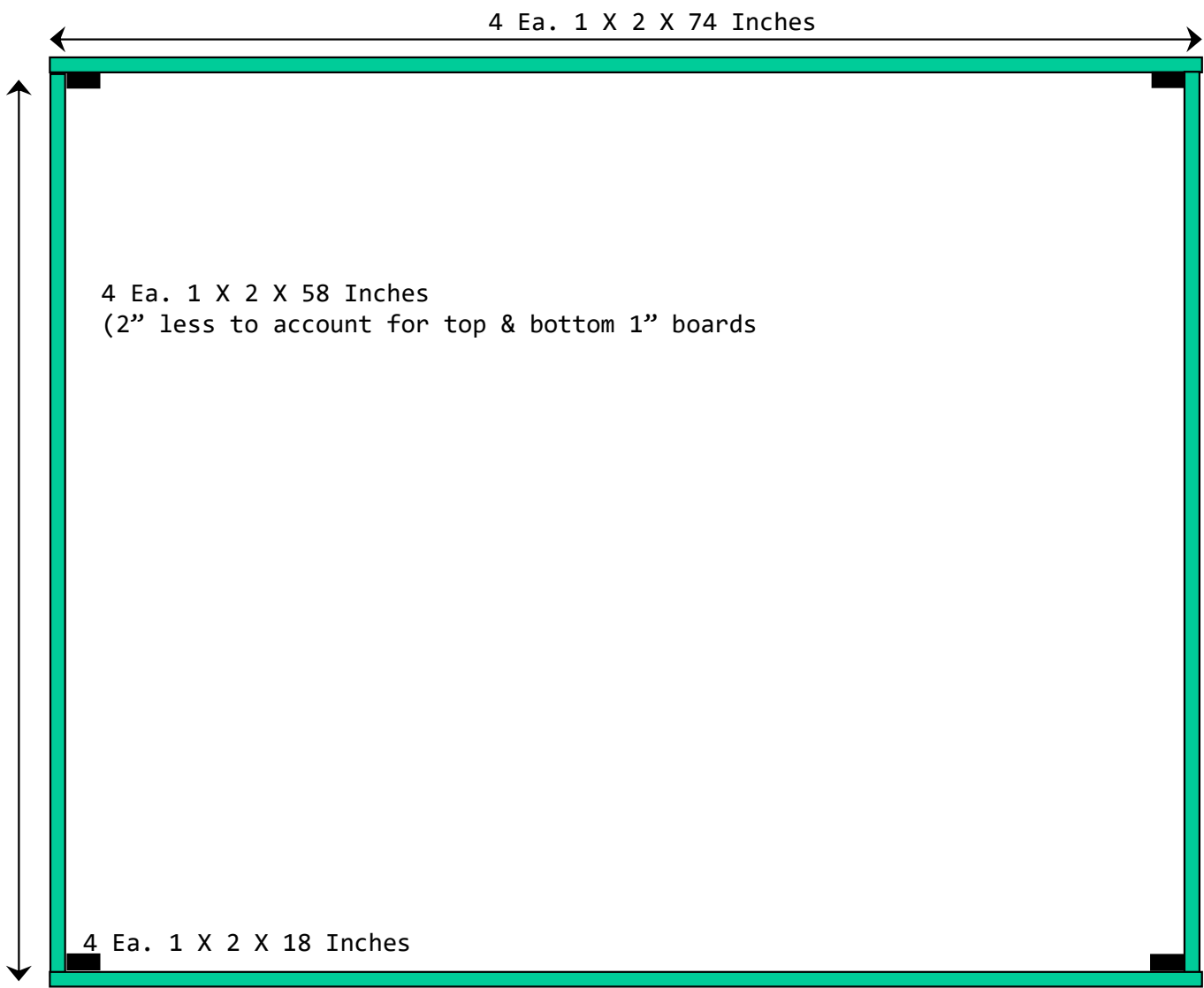
Frame #2 Top View, 2 Ea. Top and Bottom Frame
