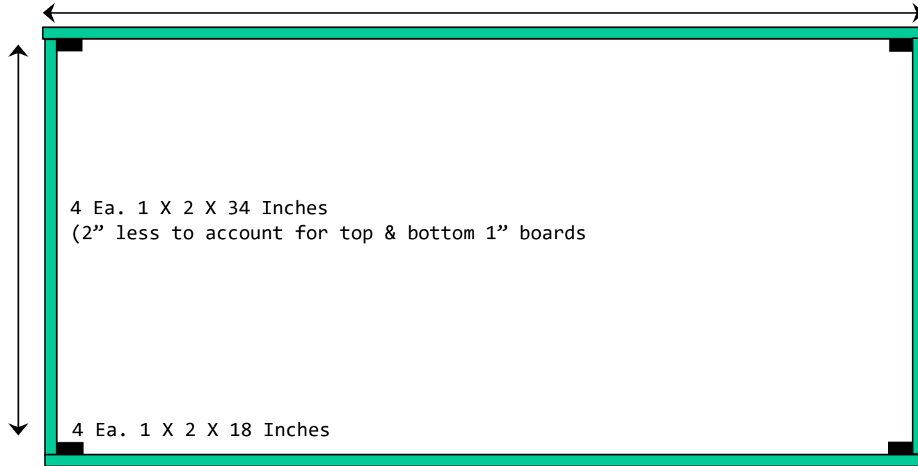
Frame #3 Top View, 2 Ea. Top and Bottom Frame 4 Ea. 1 X 2 X 72 Inches
